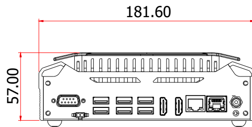
Rear View
