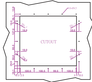
CUT OUT DIMENSION
