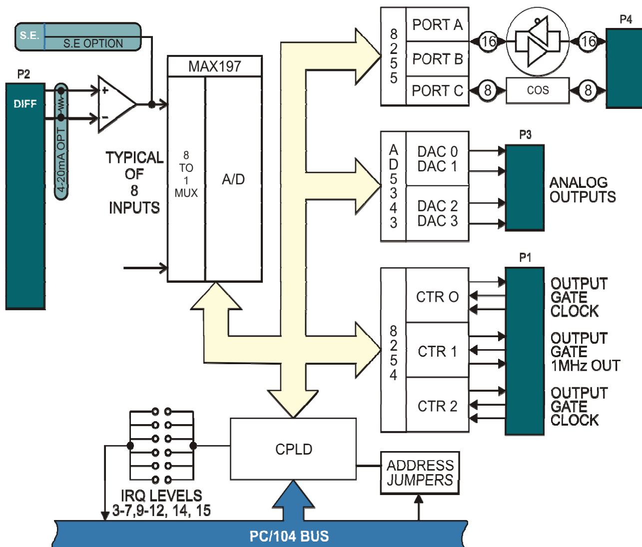
Figure 1-1: 104-AIO12-8 Analog Multifunction Board Block Diagram
