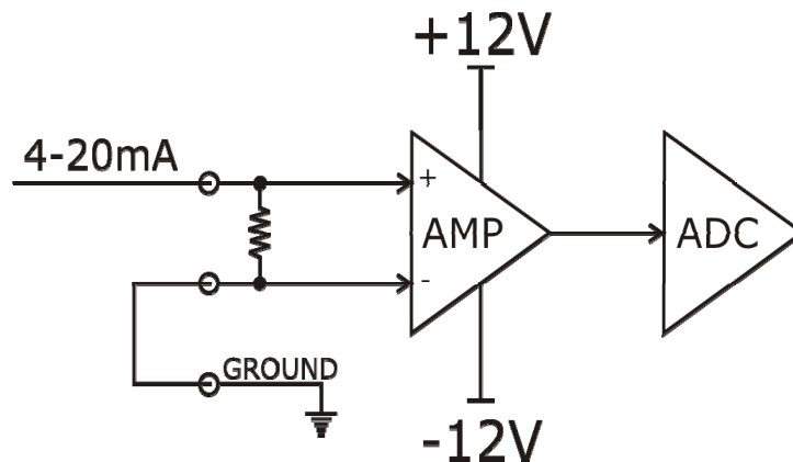
Figure 5-3: 4-20mA Source to Differential Input
