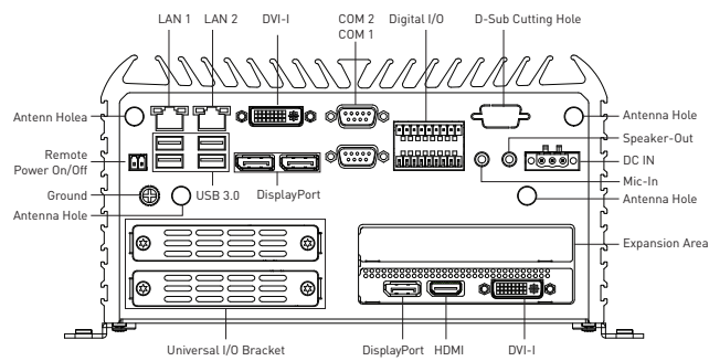
Rear Panel
