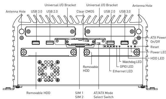
Front Panel
