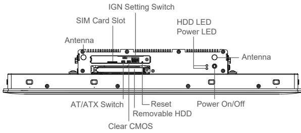
Front I/O
