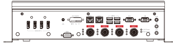
Front View (4PoEM12)
