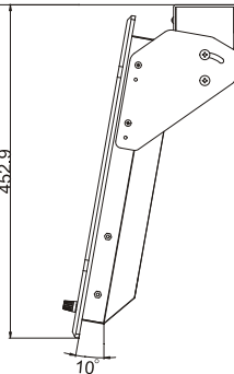
ROOF MOUNT
