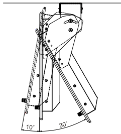
ROOF MOUNT
