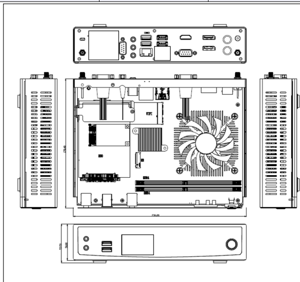
Rear Panel External I/O
