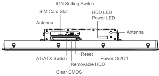
Front I/O
