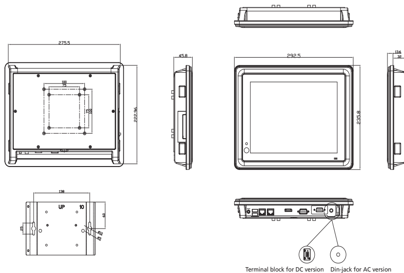
Terminal block for DC version Din-jack for AC version
