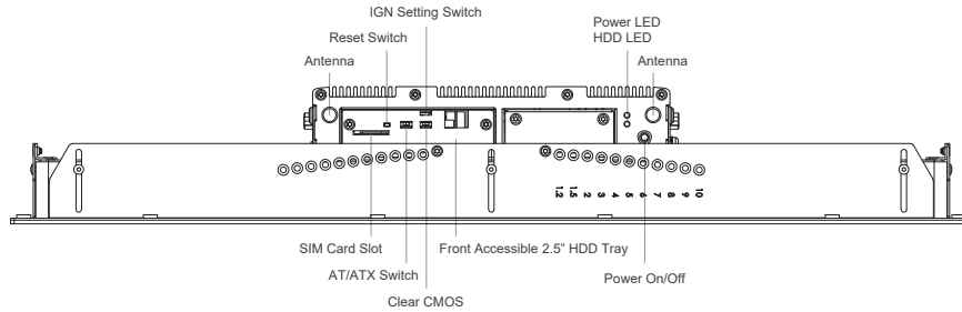
Front I/O
