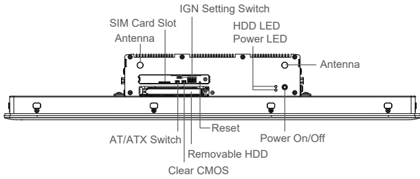
Front I/O
