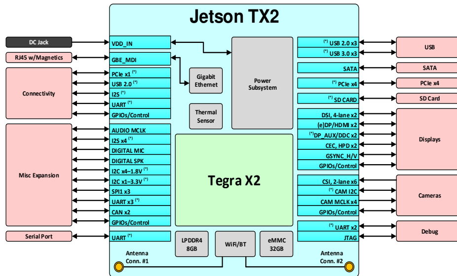
Figure 1 SOM Block Diagram – General Application
