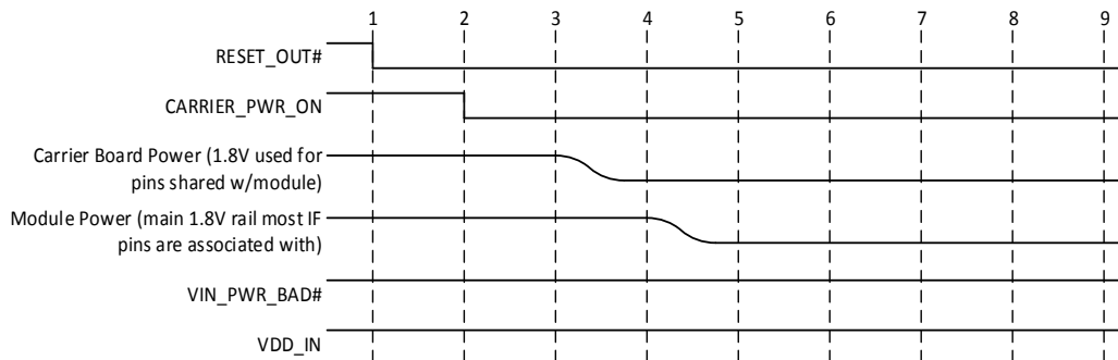
Figure 4 Power Down Sequence
