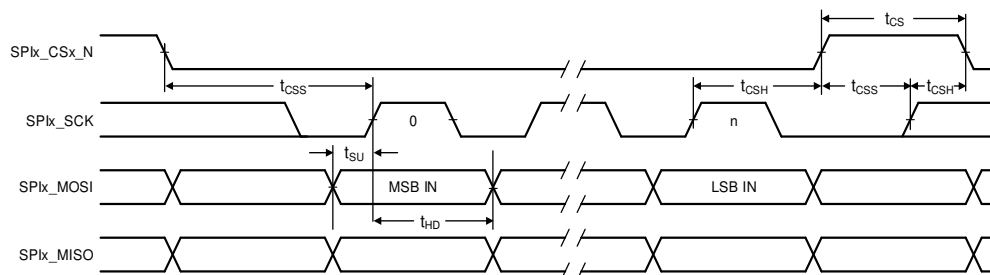
Figure 6 SPI Master Timing Diagram
