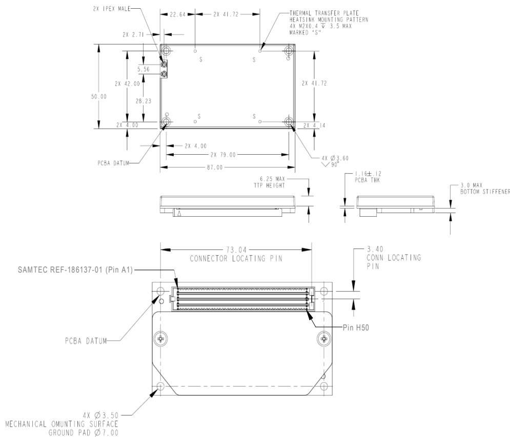
Figure 2 SOM Package Outline with Dimensions
