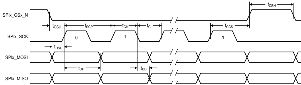
Figure 7 SPI Slave Timing Diagram
