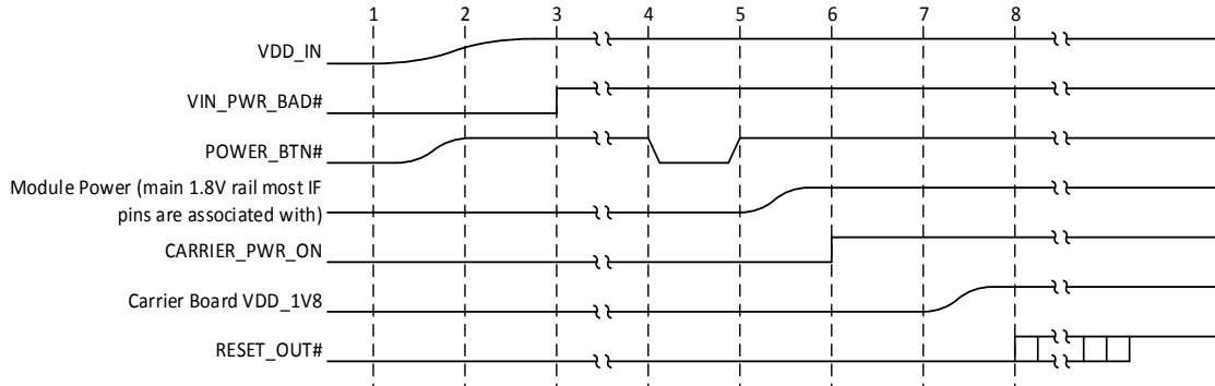
Figure 3 Power Up Sequence
