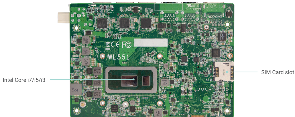
Bottom View eDP connector
