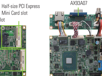
▲ Assembly view
