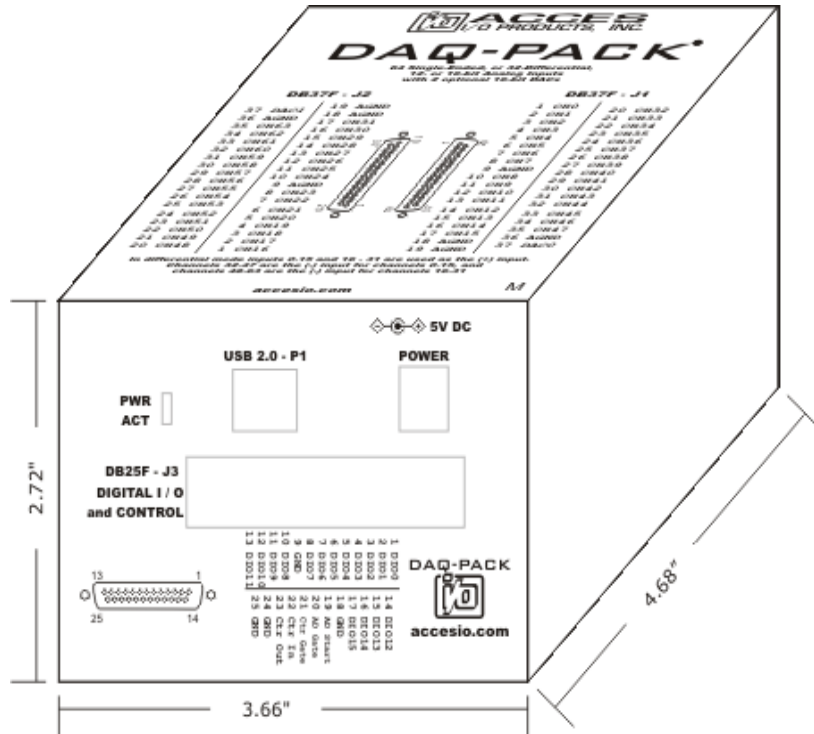
Figure 2-1: DAQ-PACK M Series Enclosure
