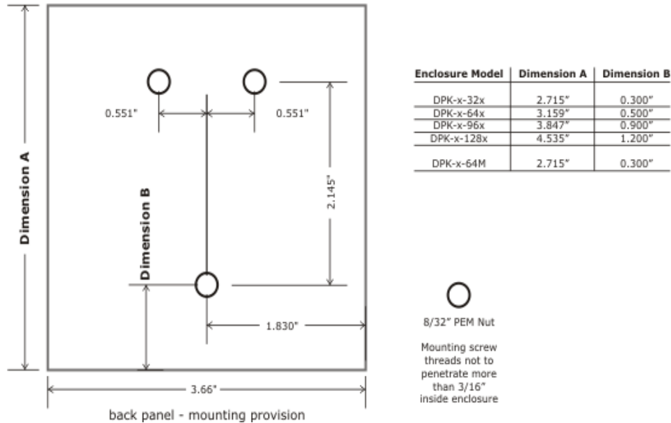
Figure 2-2: DAQ-PACK Mounting Provisions
