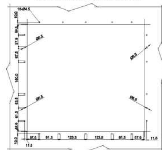
All Dimensions are ±0.5 mm
