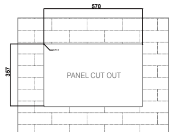
CUT OUT DIMENSION
