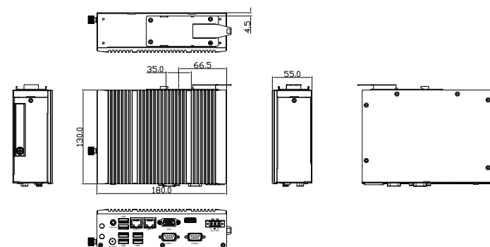
ACS-2311_DIN RAIL
