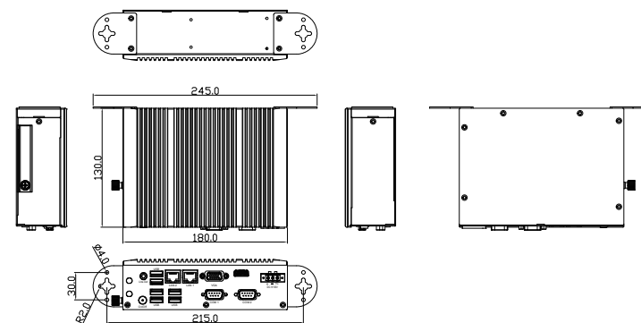
ACS-2311_DIN RAIL
