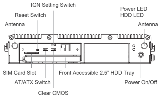
Front I/O
