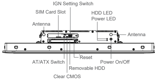
Front I/O
