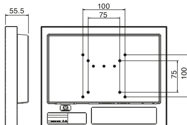
FDSV1201-F / FDSV1201T-F
