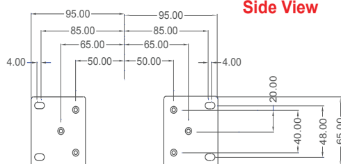
Back Plates
