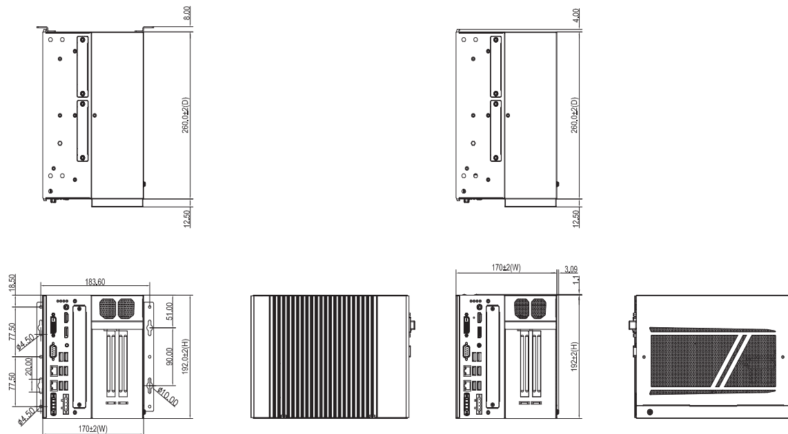
Option-wall mount
