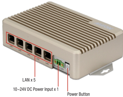
BOXER-8230AI-A3/JP46E-A1 Front View
