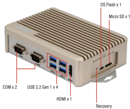
BOXER-8230AI-A4/JP46E-A2 Front View
