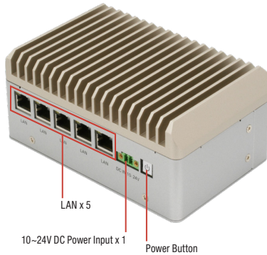
BOXER-8230AI-A4/JP46E-A2 Front View
