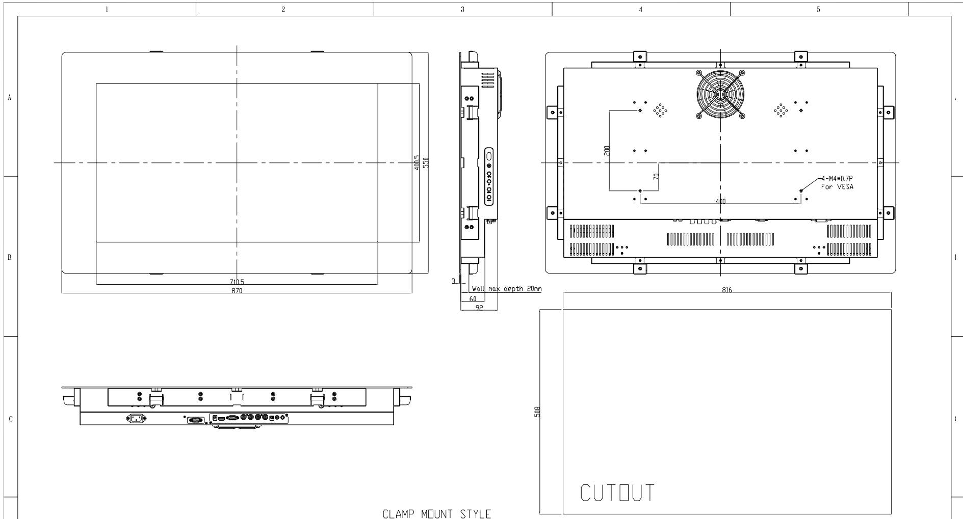
CLAMP MOUNT STYLE
