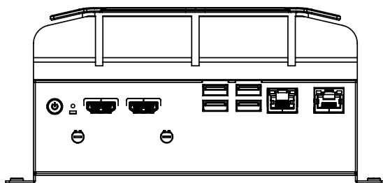
Front View ES220F-CS (3 Storage)
