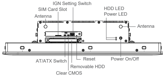
Front I/O
