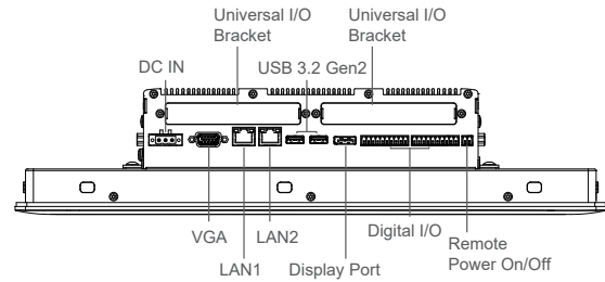
Rear I/O
