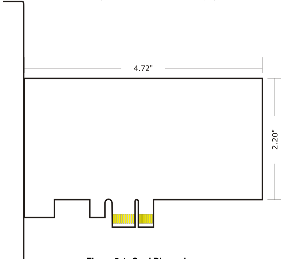
Figure 3-1: Card Dimensions
