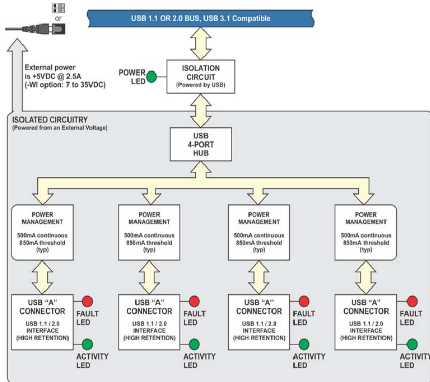
BLOCK DIAGRAM
