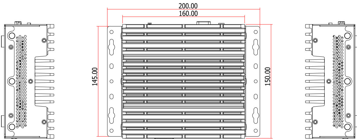
Left View
