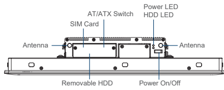
Front I/O
