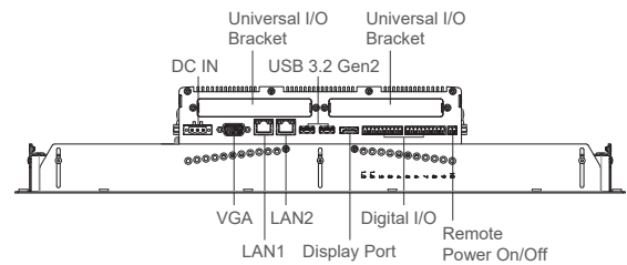
Rear I/O
