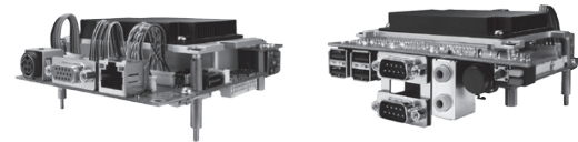
▲ Assembly view
