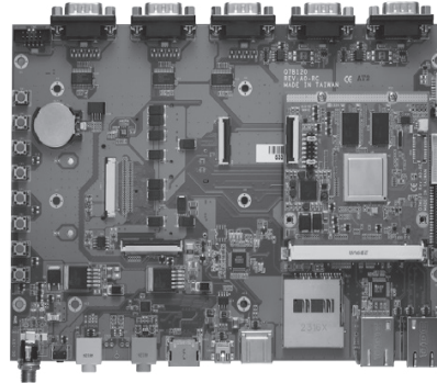
▲ Q7M120-120-EVK
