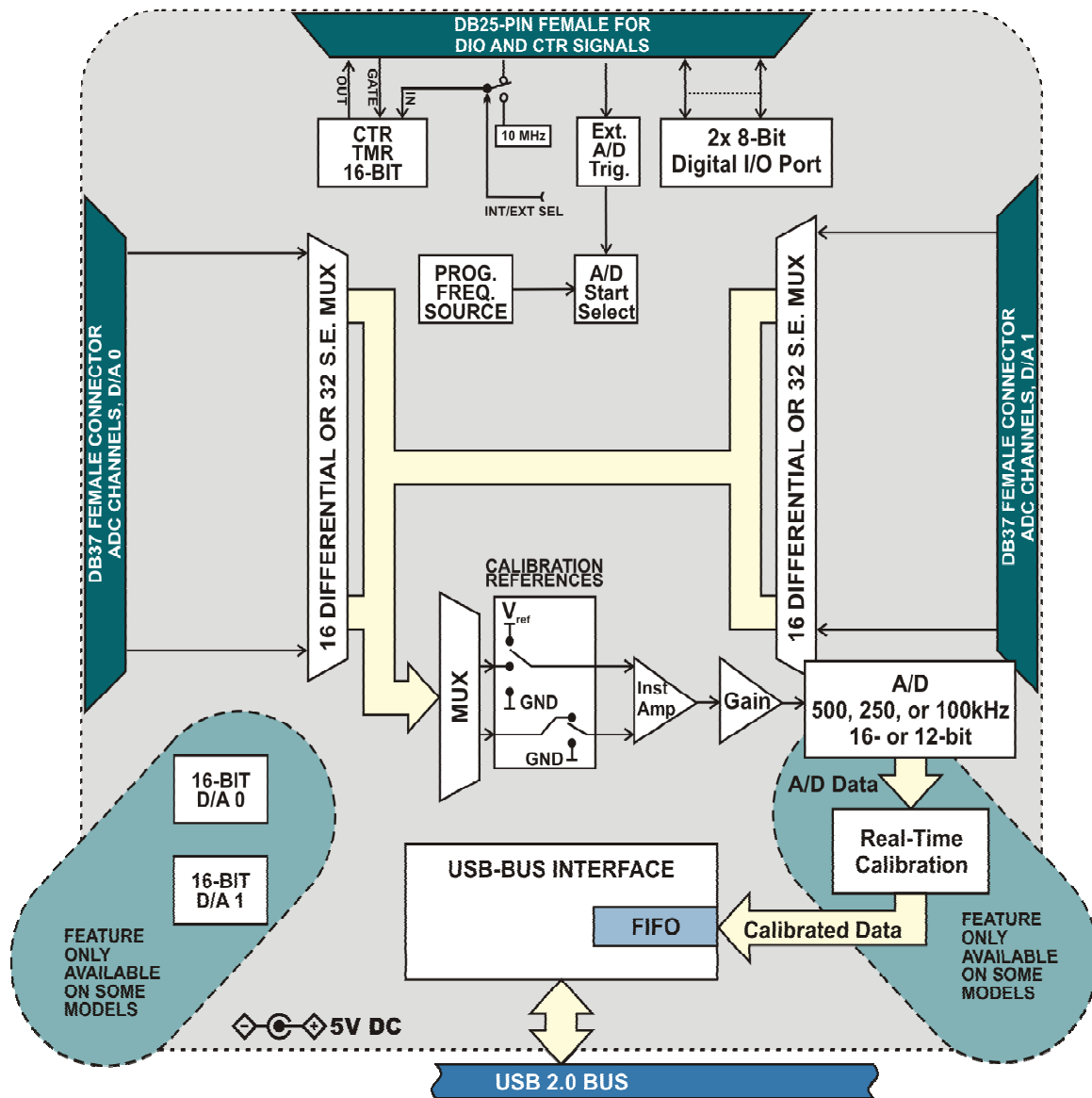
Figure 1-1: Block Diagram
